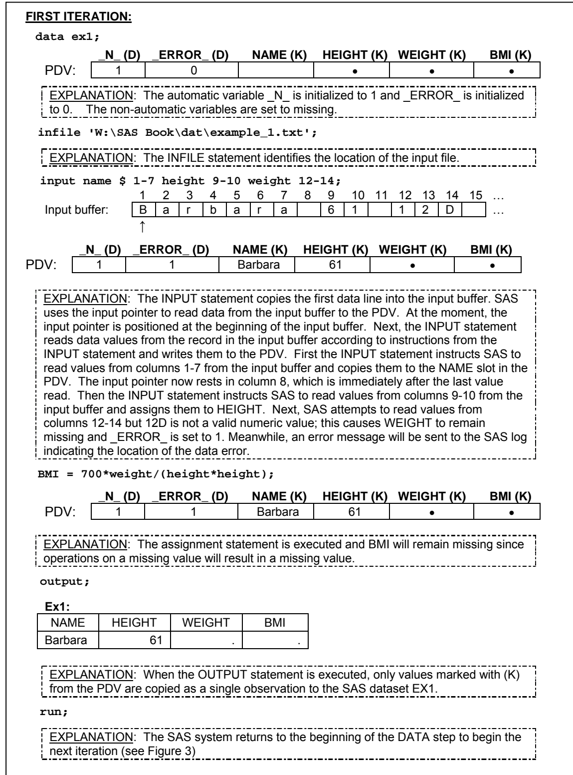
Figure 2. The first iteration of Program 1.
