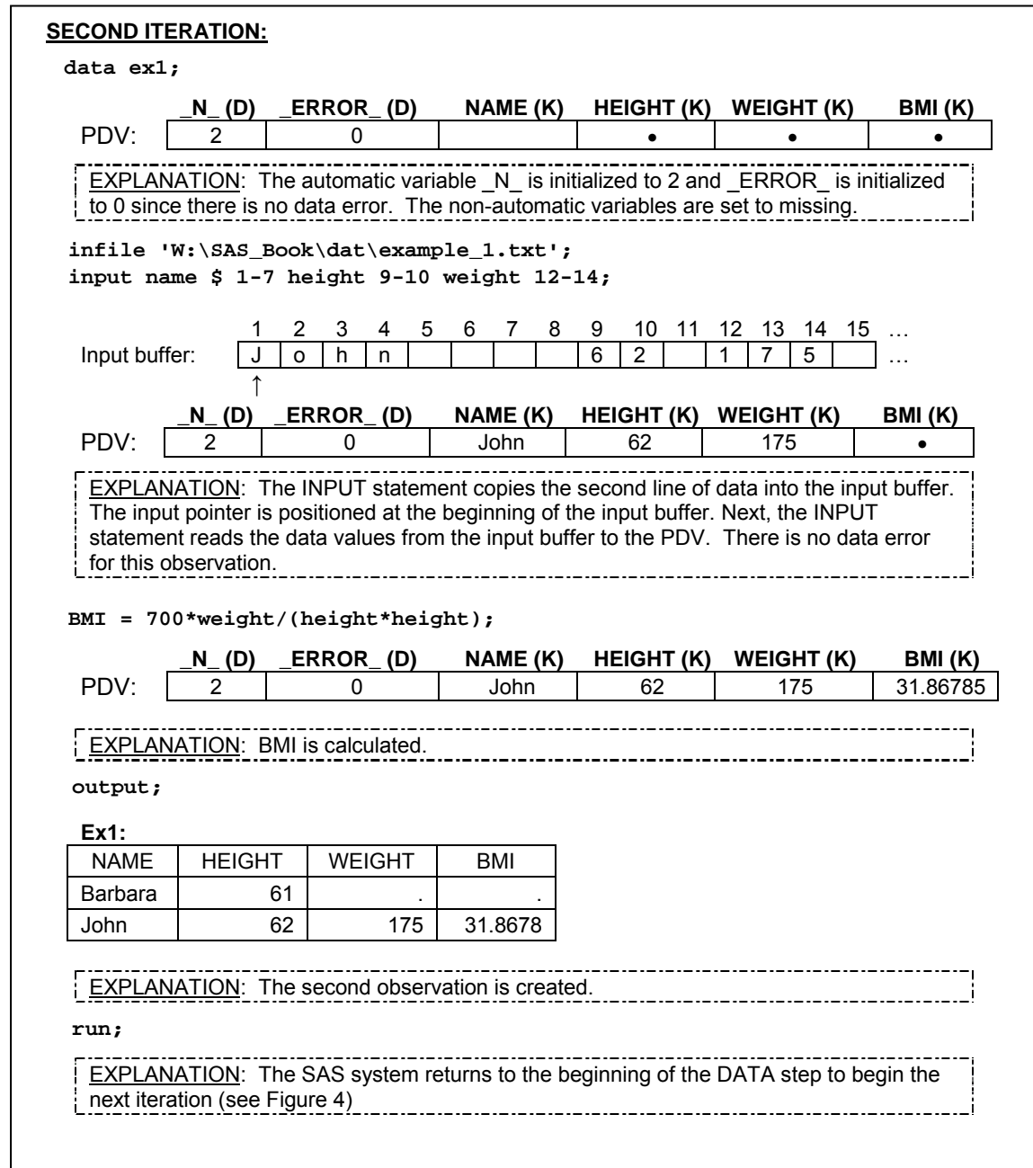
Figure 3. The second iteration of Program 1.
