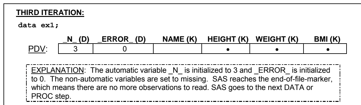
Figure 4. The third iteration of Program 1.
